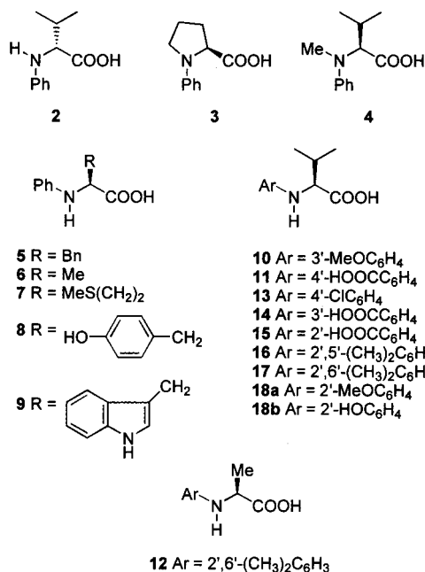
Figure 2. Structures of the coupling products catalyzed by CuI.
