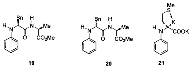
Figure 3. Structures of dipeptides 19 and 20 and potassium salt 21 .
